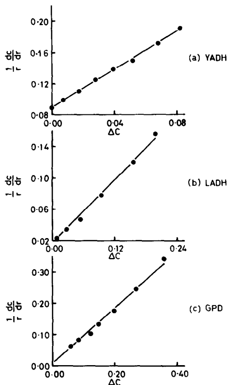
Fig. 2. Sedimentation equilibrium of maleylated, carboxy-methylated enzymes in 0.5% (w/v) ammonium hydrogen carbonate, 0.4 N sodium chloride at 20°. Concentration (c) in arbitrary units. (a) yeast alcohol dehydrogenase at 15,220 rev/min; (b) liver alcohol dehydrogenase at 12,590 rev/min; (c) pig glyceraldehyde 3-phosphate dehydrogenase at 15,220 rev/min.
